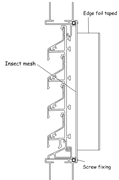
Typical demountable panel detail
