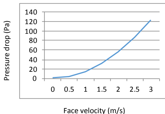
Performance: airflow, louvre with insect mesh
