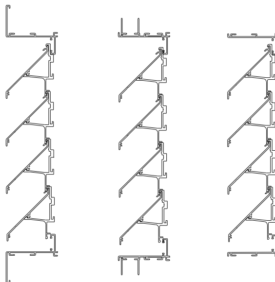
IKL751 Flange frame IKL752 Glaze in IKL753 Rebate
