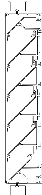
Typical detail
