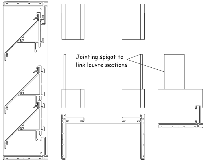
Stacking can be achieved using most outerframe sections
